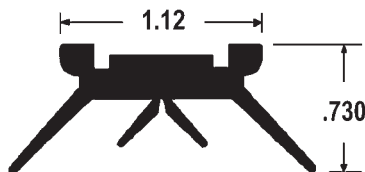
Bottom Seal WH-3765 Use with old-style 1801 Retainer
