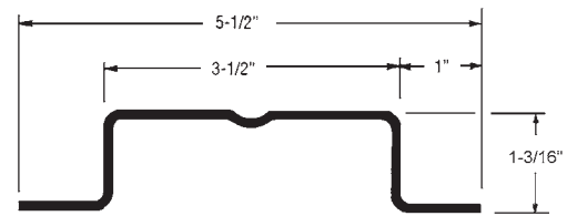
Fruehauf FR-SP03 107-1/2" 18 Ga. Galv Steel; Replaces STK-030237
