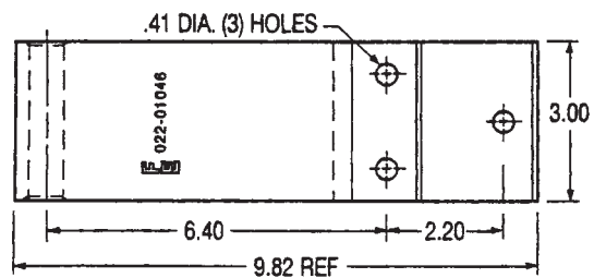
Hinge MP-HG02 004161 3-Hole
