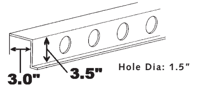
Body Rail BK-SL0853-40 240" Length 6" Hole Centers Van Sliders
