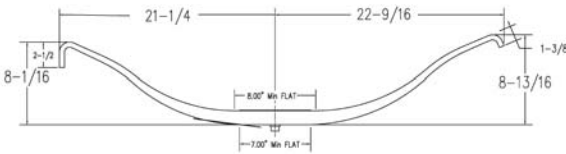
High Arch (Single Leaf) 700-3-4
