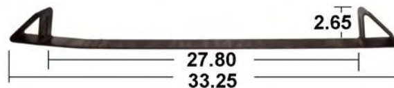
Coil Rack 700-1-67
