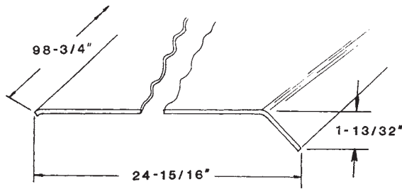
1/8" Diamond Tread Plate 523-6-722B-24 Pre-drilled for 12" crossmembers
