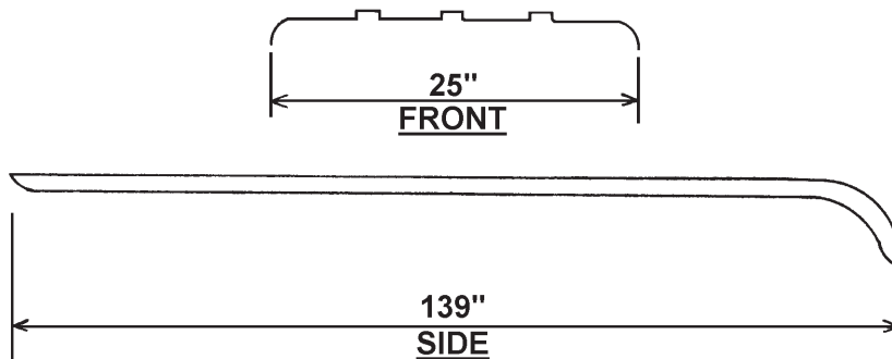
Universal Front Fender 700-99-194 .090 Aluminum
