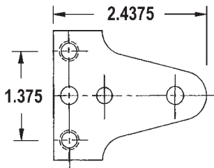
Bottom Roller Adapter Plate WH-2694
