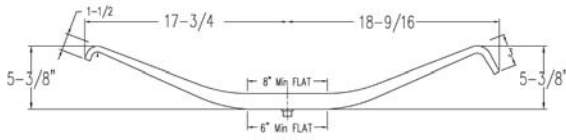
Low Arch (Single Leaf) 700-3-1
