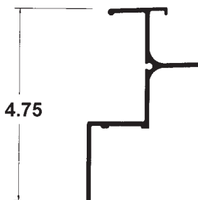
MP-000085 25'-1" Model GVFD; for 1-3/8" Roof Bows
