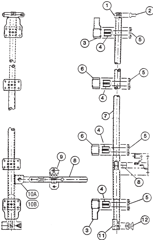
Trailmobile New Style Rear Door Lock Kit 700-532-13 Kit Components:
