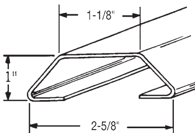
Wabash Anti-Snag WA-RB01 99" Galvanized Steel; Replaces FC#03100028
