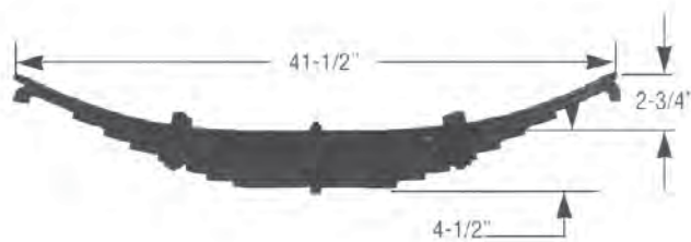
Low Arch (9 Leaf) 700-3-73 Replaces TRA696, UXA000252
