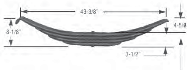
High Arch (4 Leaf) 700-3-33 Replaces TRA699, UXB000201
