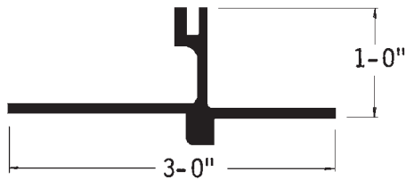
Trailmobile Side Attachment 90-4-2310-0-115 115" Aluminum
