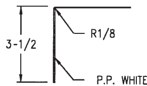
Trailmobile Reefer Inner Radius (For Standard 6" Radius) 508-15-216-22 .050 PPW Aluminum Height = 105-7/8"
