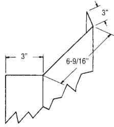
Trailmobile Dry Freight Inner Radius 9519-1-507-E9 18 Ga. Galvanized Steel Height = 108-1/8"
