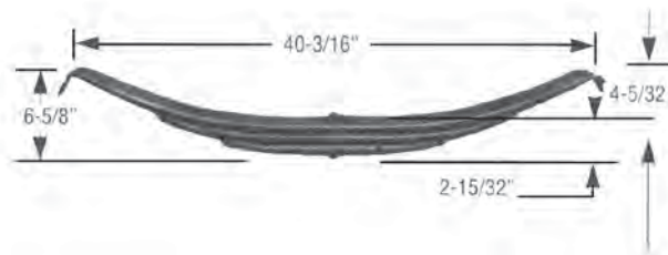
High Arch (3 Leaf) 700-3-32 Replaces TRA693, UCD0511-1
