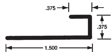
J Moulding 700-514-32 10'-0" Aluminum
