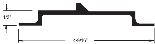
Trailmobile Side Attachment 90-4-1721-0-110 110" Aluminum
