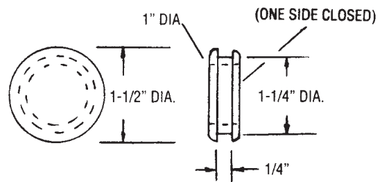
Fifth Wheel Grommet 50-14-125
