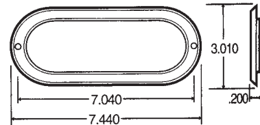
Grommet Cover TL-60703 Stainless Steel
