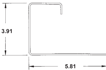
Rear Corner Post MP-1198653
