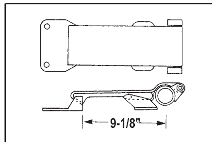
Trailmobile Mid-Cam Lock 700-532-15
