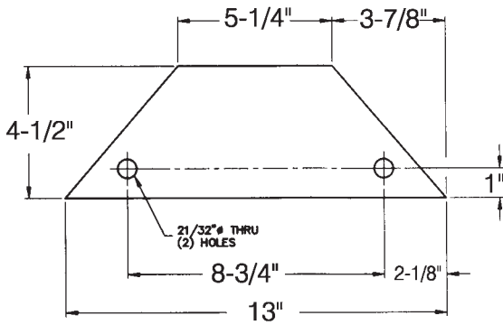
Mounting Plate 700-4-450 Replaces Great Dane 09758
