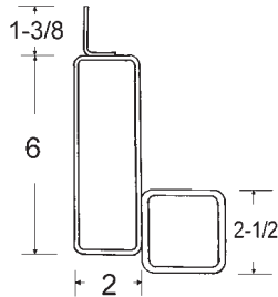
700-512-18-G 118-3/4" Galvanized Steel
