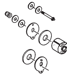
Pivot Bushing Kit DA-SR1JA112 One Side
