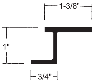
Utility UT-SP02 115" Aluminum; Replaces 1-6500-110
