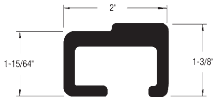
Trailmobile Reeper Composite Post Reinforcement 90-4-2107-0-16 16" Composite
