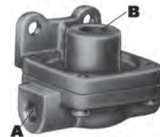
QR-1 Quick Release Valve BX-229859 AB = 3/8" Generic AV-229859
