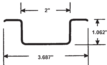
Stoughton SO-RB01 98-3/4" 3-Piece; Steel; Replaces 2306636
