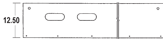
Rear Corner Post (w/ Cut Outs) MP-1198654 Curbside MP-11986540 Roadside
