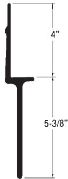
Trailmobile "Fleet" Rail 90-4-1855-559 46'-7"
