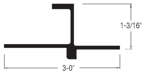
Trailmobile Side Attachment 90-4-2349-0-121 121" Aluminum
