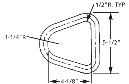
D-Ring 3/4" Dia 523-7-4 Pull Test: 57,500 to 62,500 Lbs; For 700-523-18 Retainer
