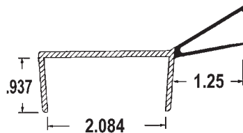
Top Seal WH-5464-96 97" For Insulated Door
