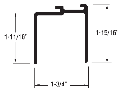
Frame Member 90-4-1727-0-104 Aluminum
