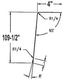
Trailmobile AddVantage Trailer Inner Radius (For 6" Radius) 519-1-1724-1196-4 18 Ga. Galvanized Steel Height = 109-1/2"
