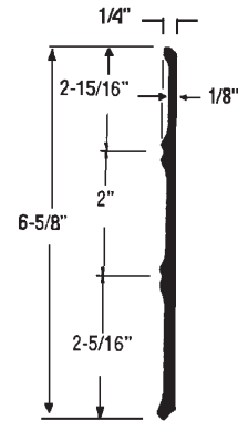
Trailmobile FRP Reinforcement 90-4-1227-553 46'-1"
