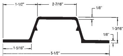
Trailmobile "O" Model 90-4-1082-0-115 115" Aluminum
