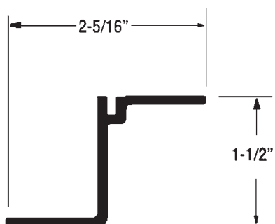
Hinge Support 90-4-1714-0-109 Aluminum
