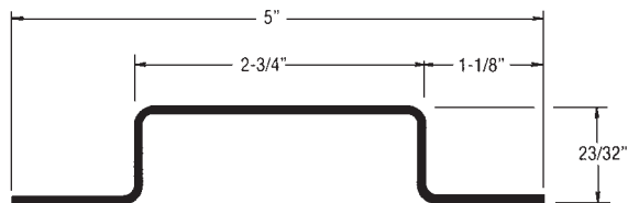
Trailmobile 90-4-2033P-0-112 112" 12 Ga. Galv. Steel; Punched
