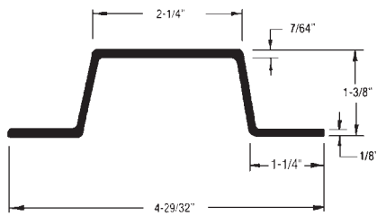
Gindy 90-4-920-0-110 110" Aluminum; Replaces GB-5
