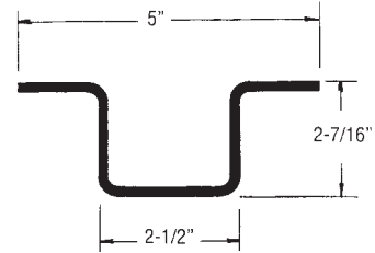
14 Ga. Galvanized Steel x 117" 90-4-2400P-0-117
