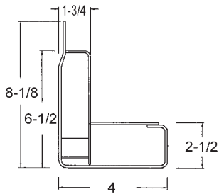
6512-A3-12L-1206-431 Roadside 6512-A3-13R-1206431A Curbside Galvanized Steel
