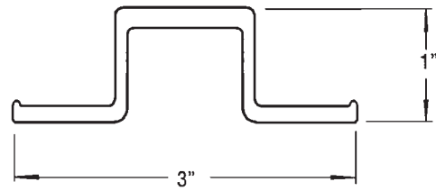
Dorsey Cambered Hat DO-RB01 98-11/16" Aluminum; Replaces 2808564
