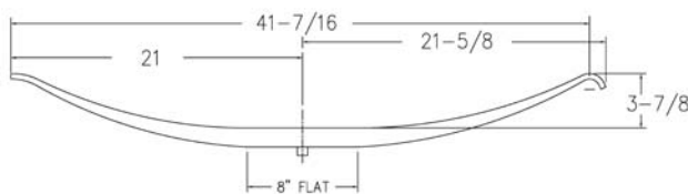
Medium Arch (Single Leaf)
