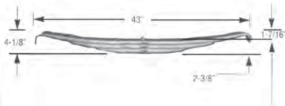
Low Arch (3 Leaf) 700-3-35 Replaces TRA697, UAC007981-001
