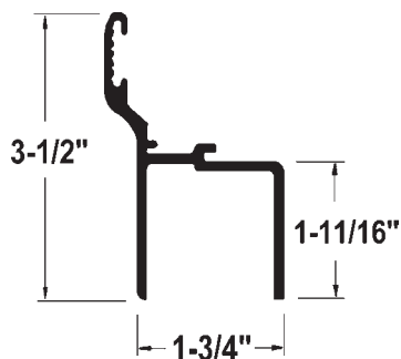
Seal Retainer 90-4-1726-0-160 Aluminum
