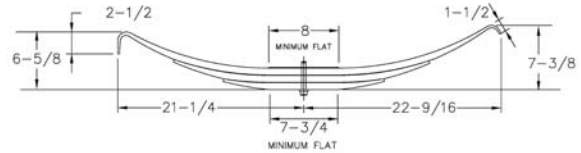
High Arch (3 Leaf) 700-3-6
