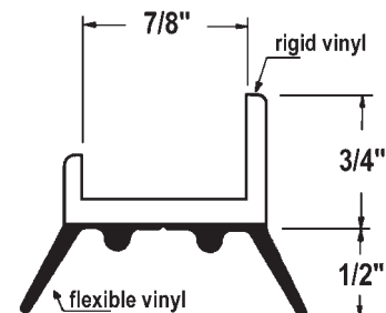
Quick Change Bottom Seal TO-70337
