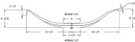
High Arch (2 Leaf) 3-A3-80
