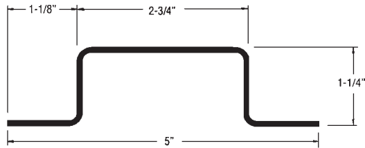
Trailmobile "A" and "D" Model 90-4-983-0-123 123" 14 Ga. Steel
