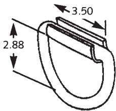
D-Ring and Retainer 5/8" Dia 700-523-7
