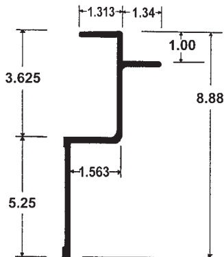
Great Dane P-Series GD-TR03-626 52'-2" Replaces AE1P0005205
