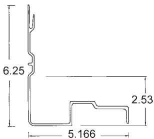
Aluminum Edge Board 90-4-2159-618 51'-6"
