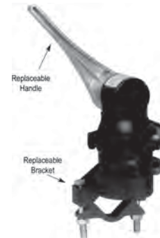
Hand Control Valve NE-90054082
