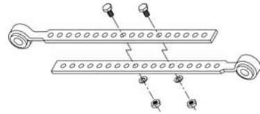
Link Assembly (Bolted) HT-A-14187
