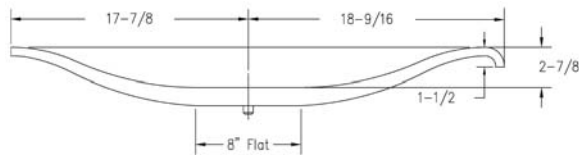
Medium Arch (Single Leaf)
