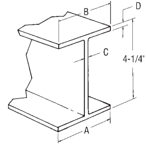
4-1/4" Aluminum 90-4-1608-0-101 Length = 100-13/16" A = 2-3/4"; B = 2-3/4"; C = .135"; D = .235"
