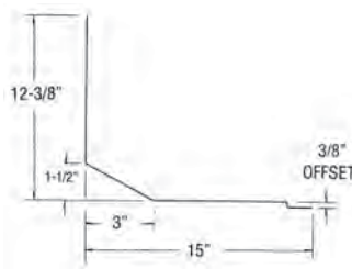
Trailmobile "A" & "D" Model Inner Radius 700-519-1 22 Ga. Galvanized Steel Height 102-1/8"
