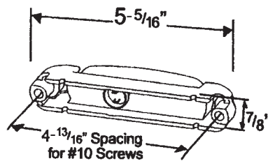
(white body) GR-46902 Red GR-46903 Amber (red body) GR-46922 Red
