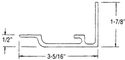
Rear Header Slam Block 90-4-1776-0-98 Aluminum
