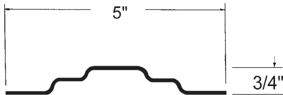
Strick "A" Slot ST-SP01 107-3/8" Steel; Replaces 46230
