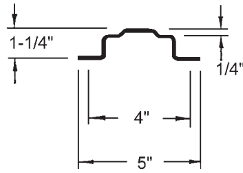
Lufkin "E" Slot LU-SP03P 115-1/4" Steel; Punched; Replaces 7087476
