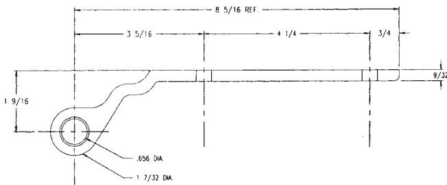
Trailmobile 4-Hole Aluminum Hinges
