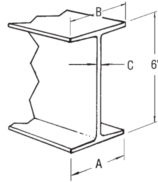
6" Steel I-Beam 90-4-1753-0-102 80,000 PSI Yield A = 2"; B = 2"; C = .106"; Length = 1-2"
