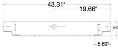
Slider Pin Cage HU-16238-05 9000 Series 44" Spring Centers
