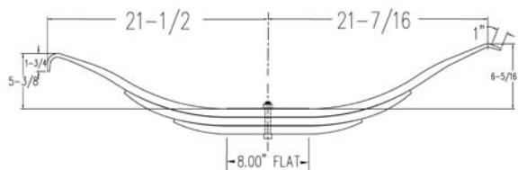
High Arch (3 Leaf)
