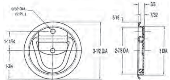
Tie-Down Ring 700-1-28 Capacity Rating: 1,200 Lbs
