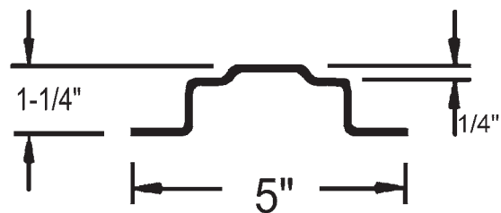
Trailmobile "E" Slot 513-5-600-1166-E-12 106-7/8" 14 Ga. Galv. Steel
