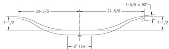
Medium Arch (Single Leaf)
