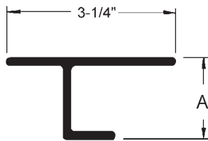
Trailmobile Reeper 90-4-1838-0-115 115"; A = 1-1/2" 90-4-1896-0-108 108"; A = 2" Composite
