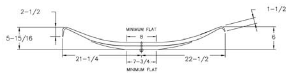
Low Arch (2 Leaf) 3-A3-83
