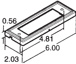
Model 21 Mounting Bracket TL-21720
