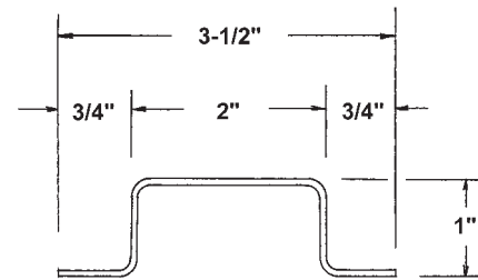
Lufkin LU-RB01 99" Galvanized Steel; Replaces 88434
