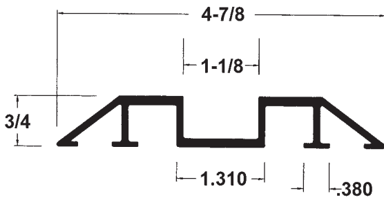
Aluminum Rub Rail 90-4-2406-621 51'-9"
