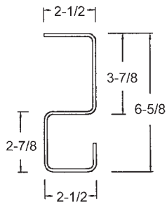
ABF w/ Roll-Up Door 6512-1-113B-4-3-L Galvanized Steel
