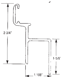
Seal Retainer 90-4-1782-0-100 Aluminum
