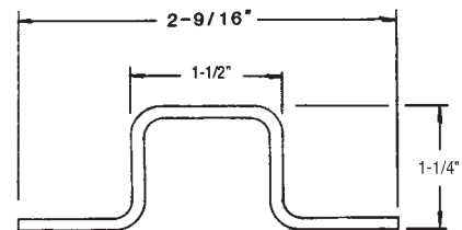
90-4-1989-553 46'-0" 12 Ga. Steel 1-1/4" Floor
