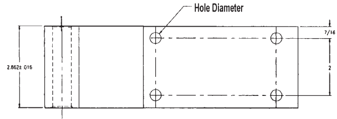
Trailmobile 4-Hole Aluminum Hinge 515-10-75
