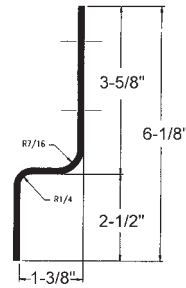
Trailmobile Top Rail Splice Inside Application for 6" Radius
