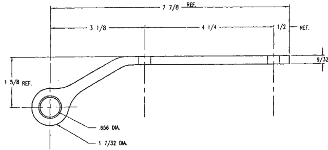
Trailmobile 4-Hole Aluminum Hinge 515-10-75
