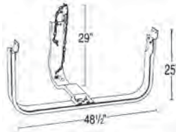
Nash Style (w/o Mounting Hardware) 700-14-3
