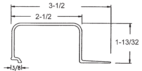
Air & Electric Channel 90-4-2309-561 46'-9"
