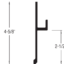
Trailmobile Side Attachment "FRP" 90-4-2173-0-115 115" Aluminum
