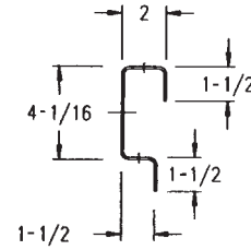
12 Ga. Steel Reinforcement Channel x 106-5/8" 511-16-566-1166
