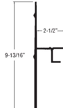
Fruehauf FB+ FR-BR03-624 52'-0" Replaces STK-020963
