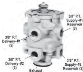
E-6 Dual Brake Valve BX-286171 Generic AV-286171
