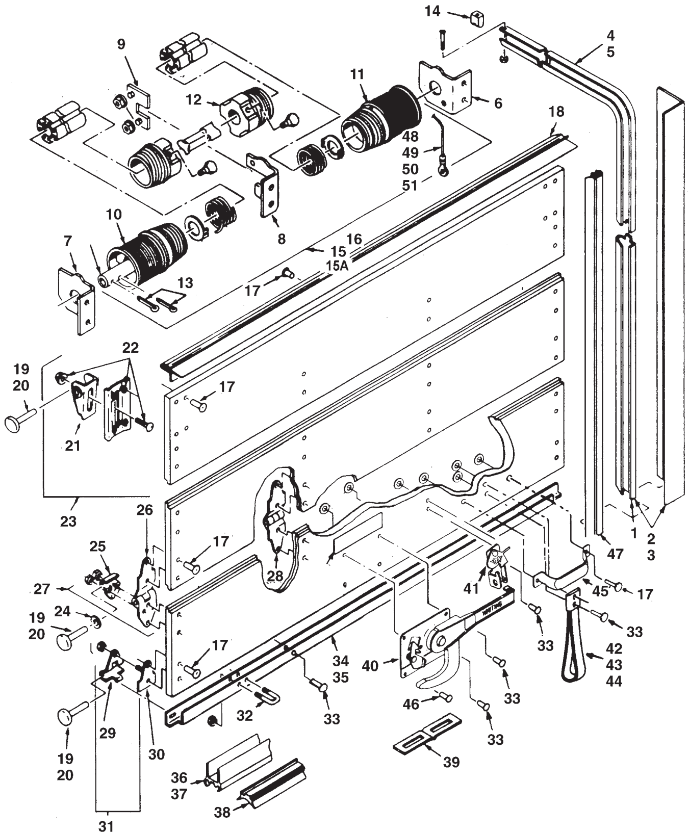
WHITING PREMIUM 3/4" DRY FREIGHT DOOR
