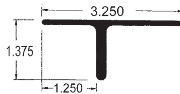
Trailmobile Reeper 90-4-2317-0-115 115" Composite
