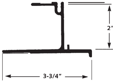
Frame Member 90-4-2216-0-120 Aluminum
