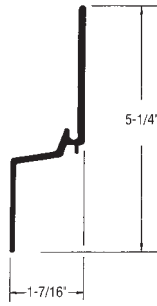
Trailmobile Top Rail Splice Outside Application 90-4-1689-108 108"
