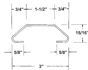
Dorsey Anti-Snag DO-RB02 98-5/8" Steel; Replaces 121069907
