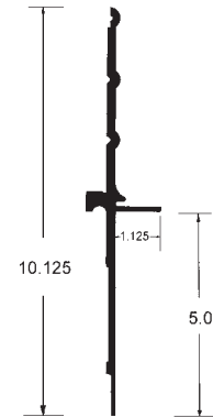
Wabash Dura Plate WA-BR04-626 52'-2" Replaces E7326260
