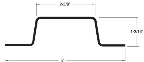
Trailmobile 90-4-1988P-0-112 112" 90-4-1988P-0-135 135" Both 16 Ga. Galv. Steel; Punched
