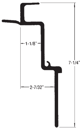
Fruehauf Double Step FR-TR04-624 52'-0" Replaces STK-021692
