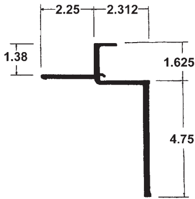
Utility 3000R UT-TR03-625 52'-1" Replaces 1-6650-150
