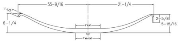
Low Arch (Single Leaf) 700-3-9
