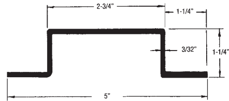
Trailmobile "A" and "D" Model 90-4-483-0-114 114" Aluminum
