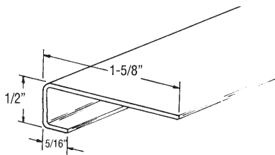
Trailmobile Nose Rail Reinforcement 90-4-1563-0-126 10'-6"; Aluminum
