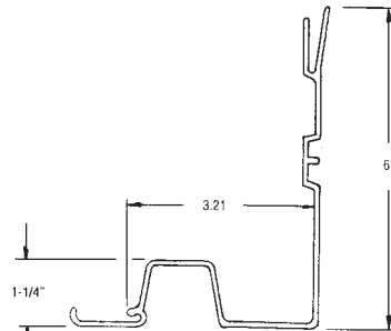
Aluminum Edge Board - Female for Corrugated Floor 90-4-1706-618 51'-6"
