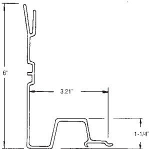
Aluminum Edge Board - Male for Corrugated Floor 90-4-1745-618 51'-6"
