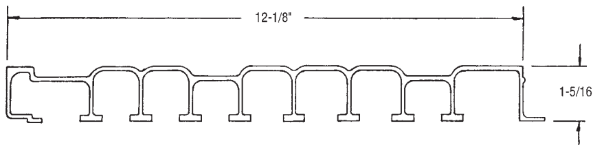
Wood Replacement Aluminum Board 90-4-2303-580 48'-4"
