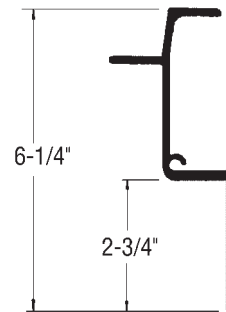
Wabash Dry Freight WA-TR01-624 52'-0" Replaces FC#08100149
