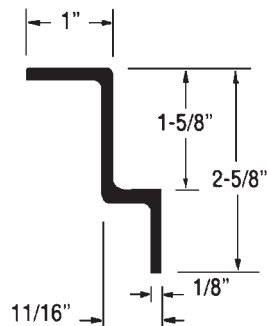
Frame Member 90-4-1728-0-108 Plastic
