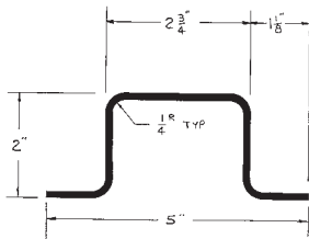
12 Ga. Galvanized Steel Shoring Channel x 94" 700-90-124 U.S. Postal Spec
