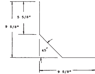
Trailmobile F.R.P. Inner Radius 9513-1-1458A 18 Ga. Galvanized Steel Height = 102-1/8"
