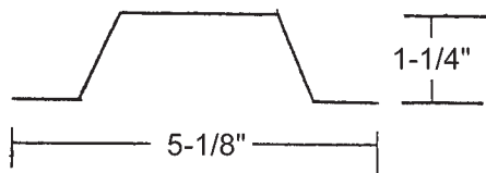
Dorsey DO-SP01 112" Steel; Replaces 1210513
