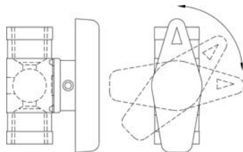
2-Way Ball Valve HT-VS-28048
