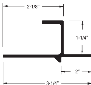
Trailmobile Side Attachment 90-4-1081-0-108 108" Aluminum
