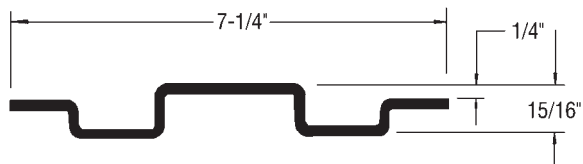
Trailmobile "E" Slot 9513-5-1114-1166-E12 106-7/8" 14 Ga. Galv. Steel
