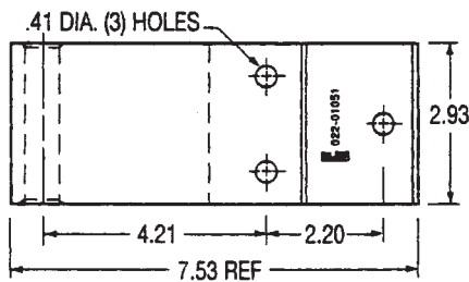
Hinge MP-HG01 004141 3-Hole
