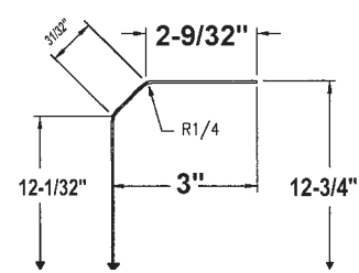
Trailmobile Dry Freight Inner Radius (For 6" Radius with 100" Inside Width) 6519-1-100-1166 18 Ga. Galvanized Steel Height = 106"
