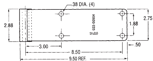
Trailmobile 4-Hole Steel Hinge 515-A10-13
