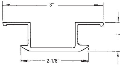
Trailmobile "A" & "D" Model Hat 90-4-703-0-93 93-1/2" Aluminum
