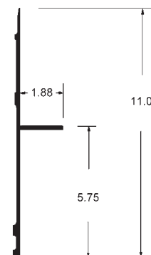
Utility 3000R UT-BR03-625 52'-1" Replaces 1-6650-149
