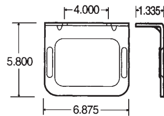
Model 45 Mounting Bracket TL-45720
