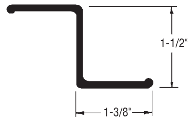
Great Dane GD-SP02 107" Aluminum; Replaces 75722
