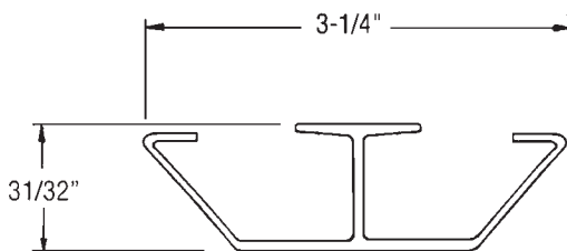
Fruehauf Cambered Anti-Snag FR-RB04 98-5/8" Replaces RCF-004335-4
