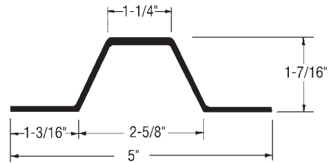
Gindy-Strick 90-4-921-0-110 110" Aluminum; Replaces GB-6
