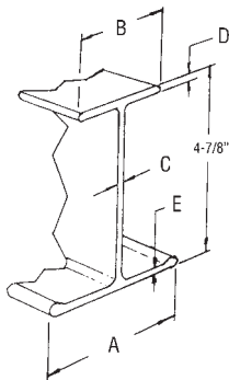
4-7/8" Aluminum 90-4-871-0-99 Length = 99" A = 2-3/4"; B = 2"; C = .125"; D = .188"; E = .156"
