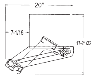
Retractable Step Assembly PZ-08-02
