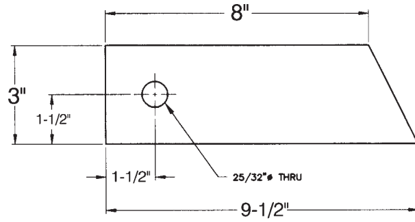
Upper Brace Lug 700-4-452 Replaces Great Dane 09955
