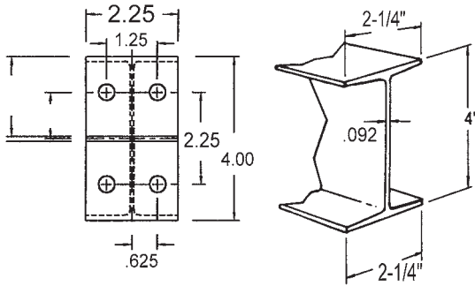
4" Steel I-Beam w/ Clip 6001-A3-101B Length = 101-5/8"
