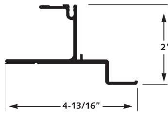
Frame Member 90-4-2225-0-165 Aluminum
