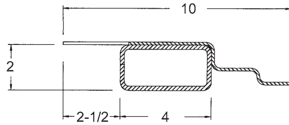
Dry Freight w/ Swing Doors 9512-A1-135B-G Galvanized Steel
