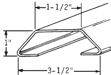
Fruehauf Anti-Snag FR-RB03 99" Aluminum; Replaces RCF-003718-1
