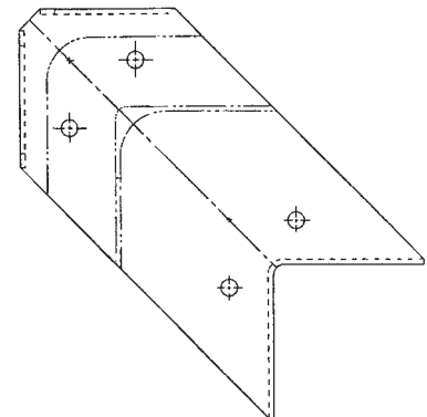
Corner Stamping 515-16-45 Aluminum
