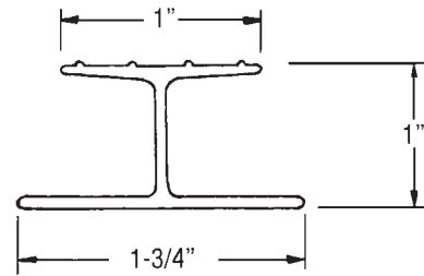
Fruehauf I Beam FR-RB01 99" Aluminum; Replaces RCC-008431
