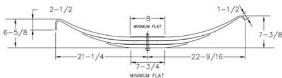
Medium Arch (3 Leaf) 700-3-7
