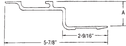
Rear Corner Post Slam Block Aluminum
