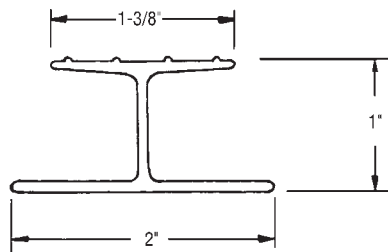
Fruehauf I Beam FR-RB02 99" Aluminum; Replaces RCF-004048-1
