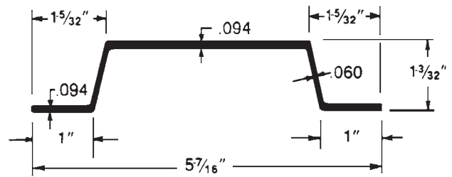
Fruehauf FR-SP01 115" Aluminum; Replaces STK-020522
