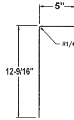
Trailmobile Dry Freight Inner Radius (For Standard 6" Radius) 9519-1-909 18 Ga. Galvanized Steel Height = 106-3/4"
