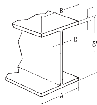
5" Aluminum 90-4-2028-0-102 Length = 101-5/8" A = 2-1/2"; B = 2-1/2"; C = .120"; D = .180"
