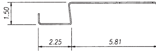
Rear Header (Upper) MP-1121823 102"
