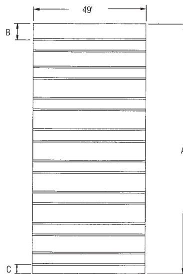
Great Dane Corrugated 4" & 8" Centers
