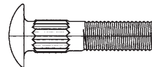
Rib Neck Step Bolts WH-10-1003-8 1/4" X 1-1/4" WH-10-1003-2 1/4" X 1-3/4"
