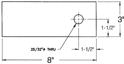
Lower Brace Lug 700-4-451 Replaces Great Dane 09954
