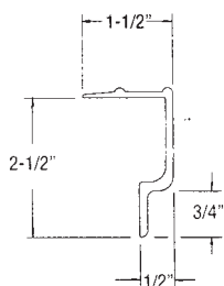
90-4-1584-0-100 For 2-1/2" Wall; Aluminum
