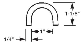
D-Ring Retainer 700-523-18 For 523-7-4 D-Ring
