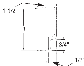
90-4-1585-0-100 For 3" Wall; Aluminum
